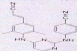
Figure 1. Chemical Structure of Rilpivirine
