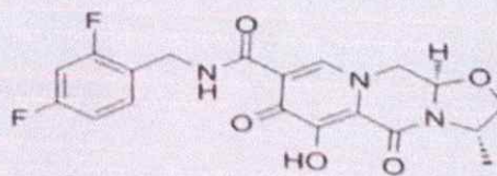
Figure 2. Chemical Structure of Cabotegravir
